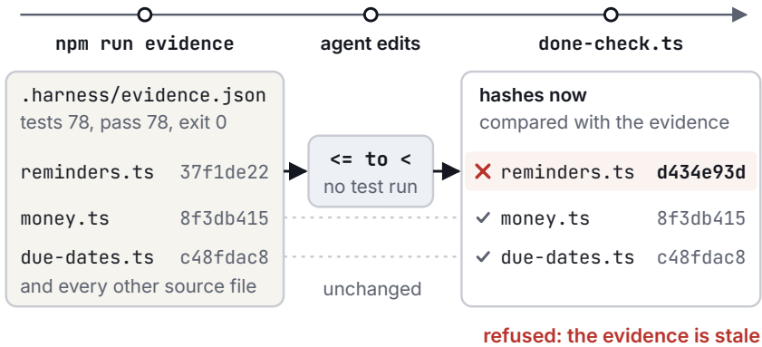
Figure 6.3. Drill D12 as a time line. The evidence file records a hash of every source file when the tests pass; the one-character edit changes the hash of reminders.ts , so done-check finds the evidence stale. Hashes are real, shortened to eight characters.
