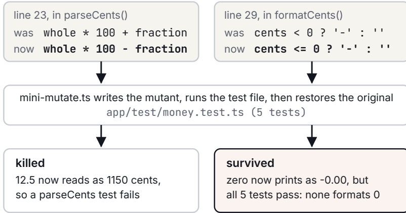
Figure 6.2. Two of the three mutants of money.ts , judged by the same five tests. A test fails on the first, so it is killed; the second changes how zero prints and every test still passes, so it survives and points at a missing assertion.
