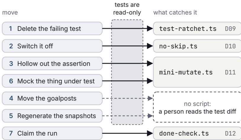
Figure 6.1. The seven moves and what catches each in Invoicer, with the drill that proves it. Moves 1 to 6 all edit a test file, so the read-only rule meets them first; permissions leak, so each still needs something behind it, and for moves 4 and 5 that is a person reading the diff.
